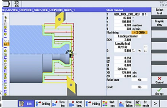
Cycle952 now also allows for four-axis chip removal on multi-channel turning machines
