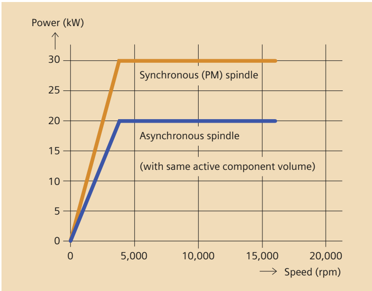
With the same active part volume and the same rated current, PM synchronous spindles have a higher power density than asynchronous spindles and allow for greater torque efficiency
