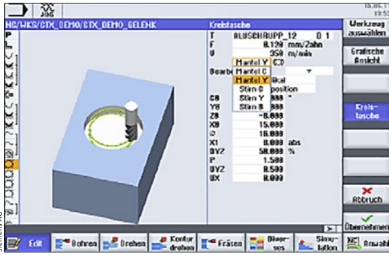
All milling cycles on the turning machine are identical to those in ShopMill
