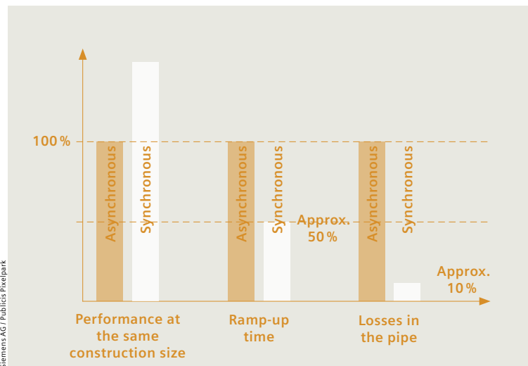
Permanent-magnet (PM) synchronous spindles are increasingly used even in standard machines due to their productivity advantages
